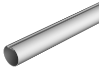
Tube T-004 Spec: Ø38mm | 1 1/2" Thickness: 2.0mm Material: Alu Color: Alu
