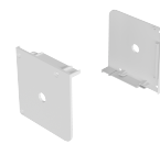
Side Caps P-I-235A-A01/A02 Spec: 88*88mm | 3 1/2" * 3 1/2" Material: PA6+15%GF Color: Four colors
