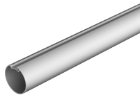
Tube T-004 Spec: ∅38mm | 1 1/2" Thickness: 2.0mm Material: Alu Color: Alu
